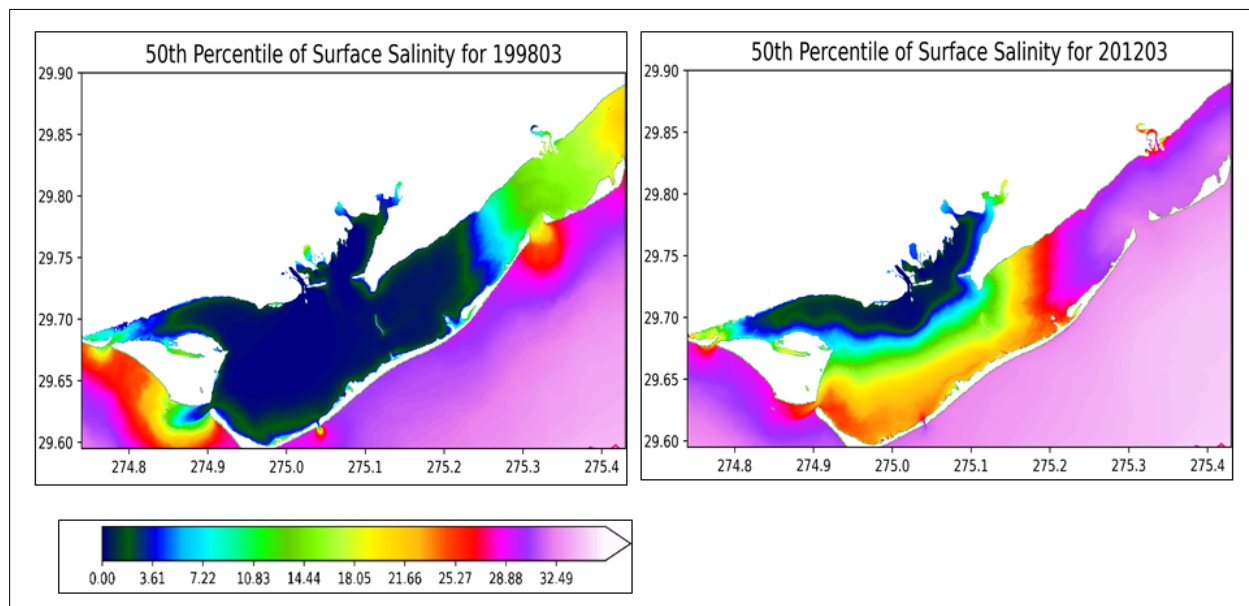
Figure 5. Maps of median salinity for March 1998 (left – a month with anomalously high river discharge) and March 2012 (right – a month with anomalously low river discharge)
