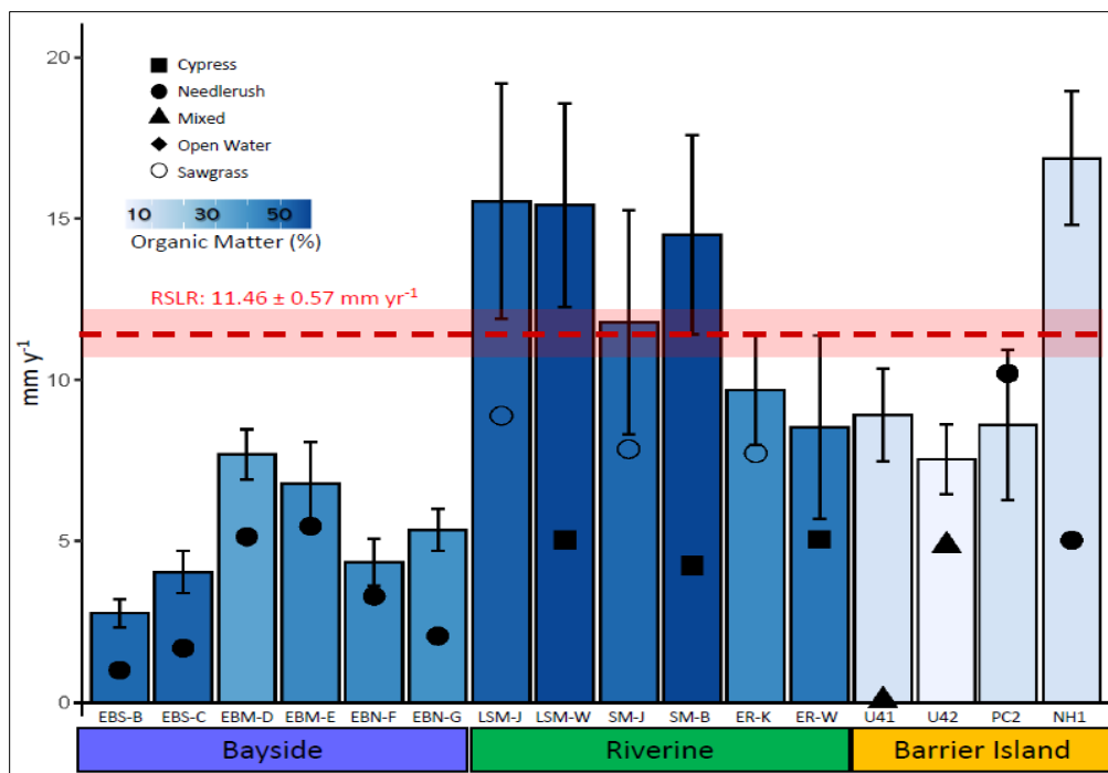
Figure 36. Average accretion rates (mm y -1 ) at each site (bars) colored by organic matter content and average rates of elevation change per SET (mm y -1 , points). Shape of points indicate dominant vegetation type at each SET. Horizontal dotted red line and shading represents the calculated rate of relative sea-level rise between 2010-2021 ± standard error.
