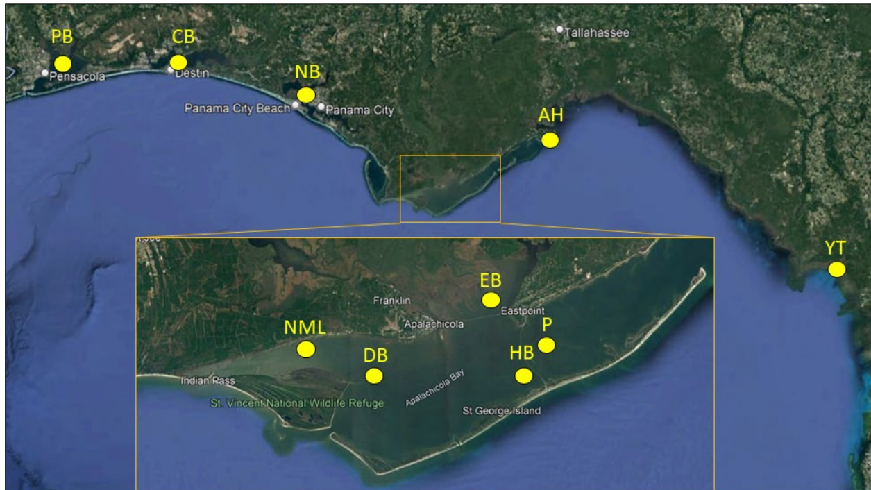
Figure 6. Map of oyster populations sampled in the Gulf of Mexico. PB = Pensacola Bay, CB = Choctawatchee Bay, NB = St. Andrews Bay North, NML = Nine Mile Lump, DB = Dry Bar, EB = East Bay, P = Platform, HB = Hotel Bar, AH, Alligator Harbor, YT = Yankee Town.
